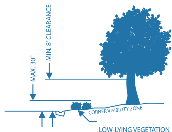
TRIMMING DETAIL
