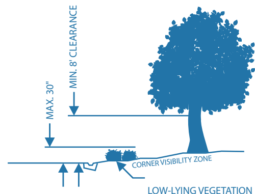
TRIMMING DETAIL
